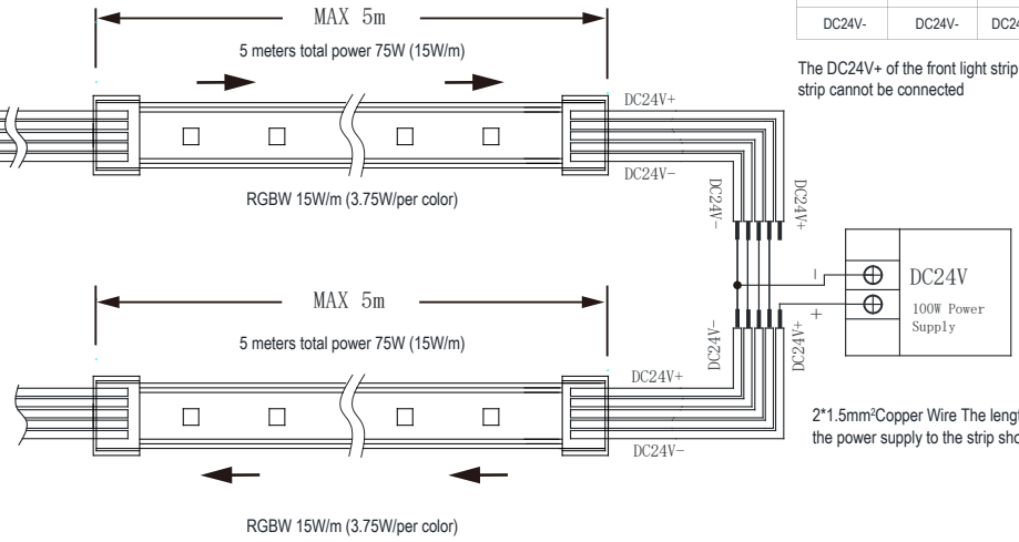
Wire Illustration among power supply, controller and strip light
